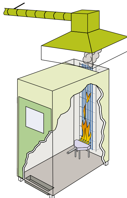
Figure 10: FTT EN 60332-3 Vertical Flame Propagation Test for vertically mounted bunched cables
