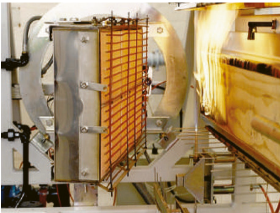
Panel box assembly with reverberatory screen as mounted in equipment test frame.
