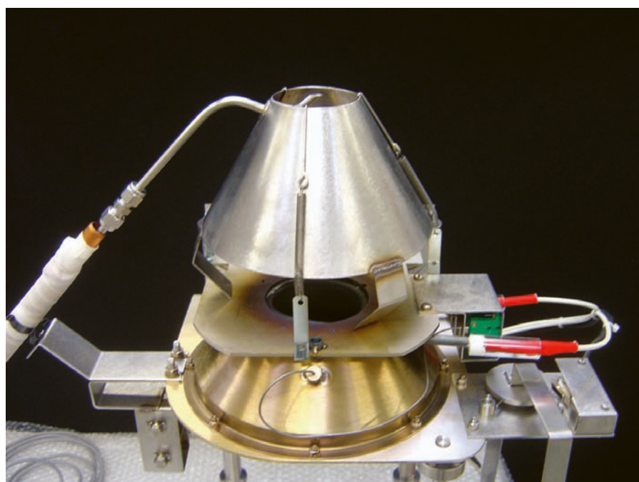
Cone Corrosimeter
