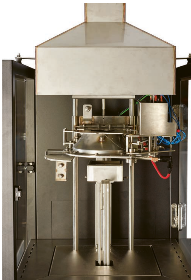
Fire model and specimen inside glass protective screen
