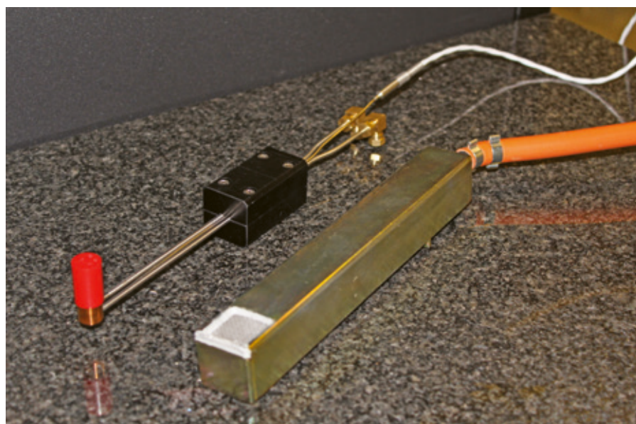
Heat flux meter and calibration burner
